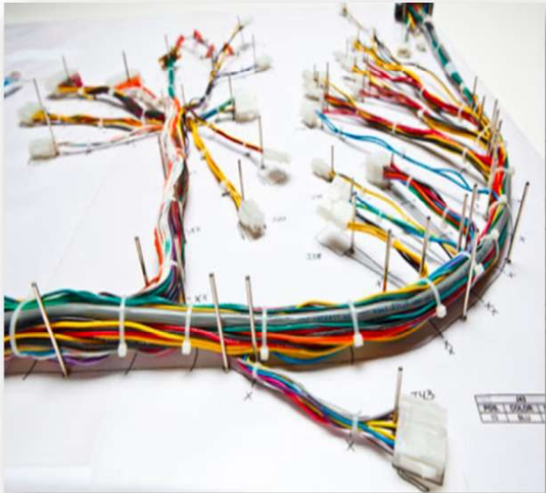
Wiring Harnesses
