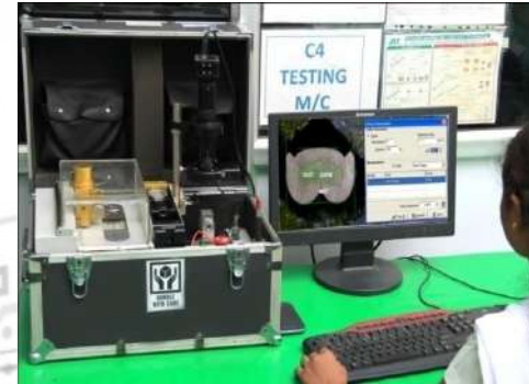
Crimp Profile Projector/Crimp Validation Equipment
